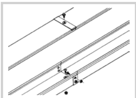
JONCTION ENTRE ACCESSOIRE ET ACCESSOIRE COUPLING BETWEEN FITTINGS
